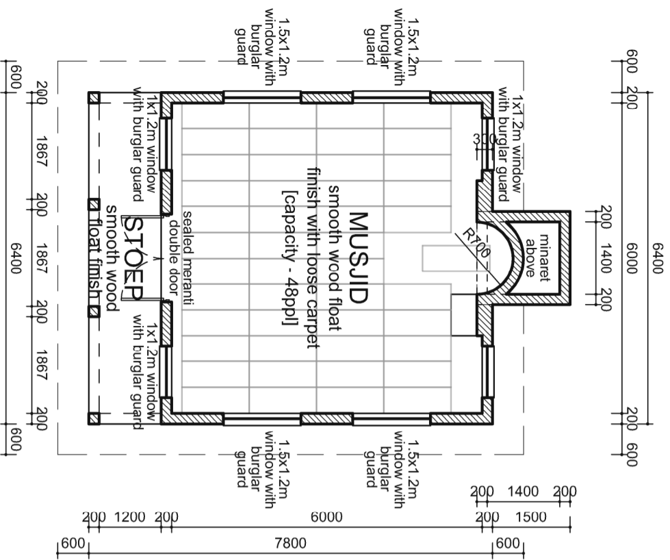
MUSJID PLAN
