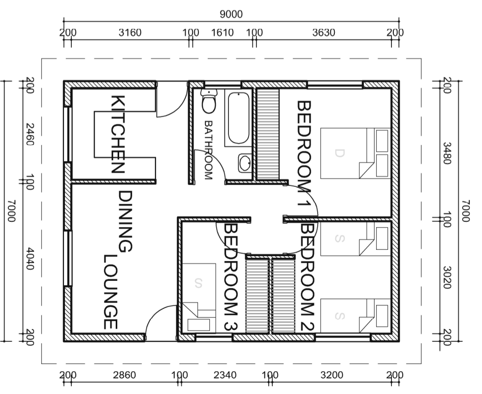
HOUSE PLAN
