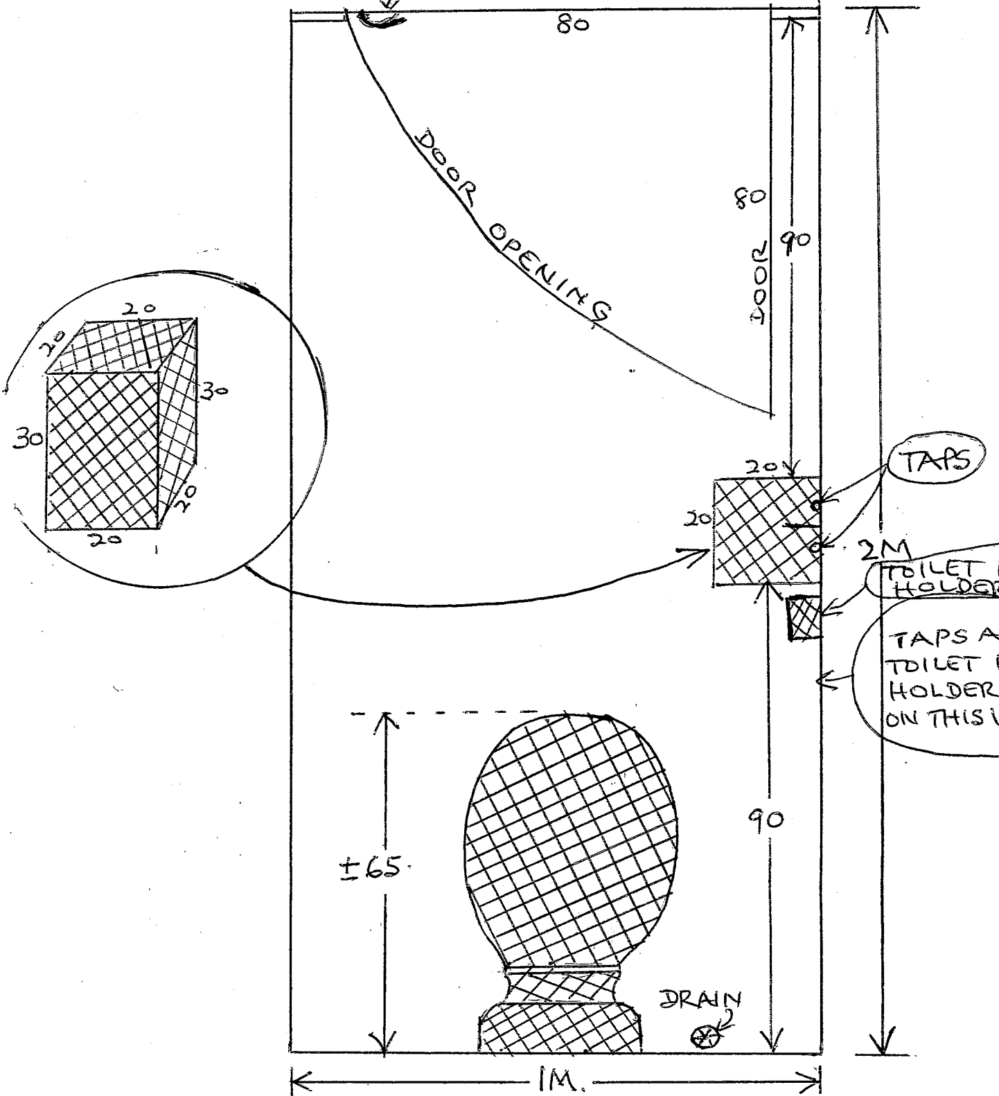
SUGGESTED TOILET PLAN FOR HIGH-PAN TOILET AERIAL VIEW
