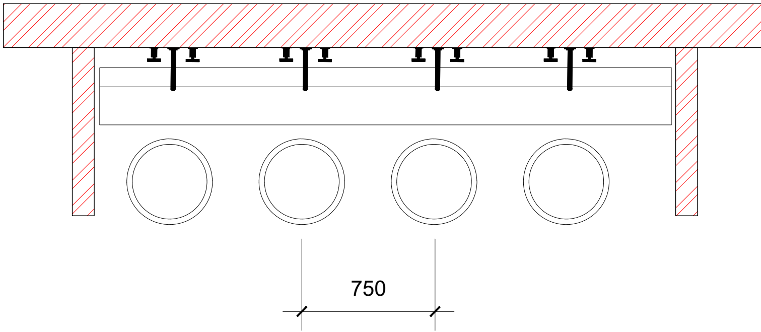
PLAN SHOWING PART WUDU AREA SCALE 1:20
